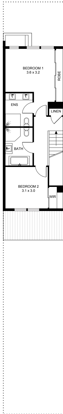
FIRST FLOOR
